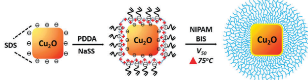
Scheme 2 Schematic illustration of the synthesis procedure of Cu 2 O@PNIPAM core-shell nanoparticles.
