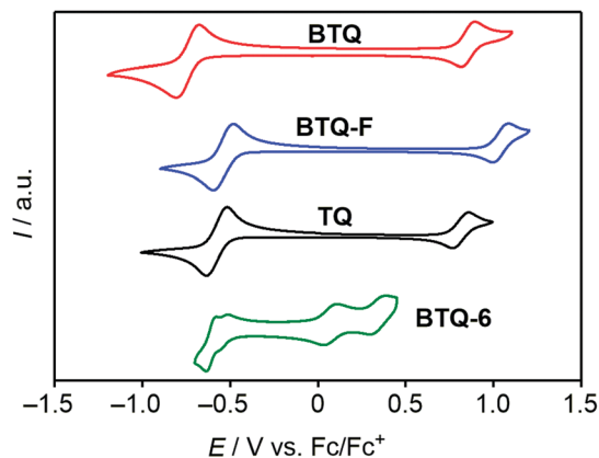
Fig. 4 Cyclic voltammograms of BTQ (red) and BTQ-F (blue), TQ (black), and BTQ-6 (green) in \text{CH}_2\text{Cl}_2 containing 0.1 M \text{TBAPF}_6 .
