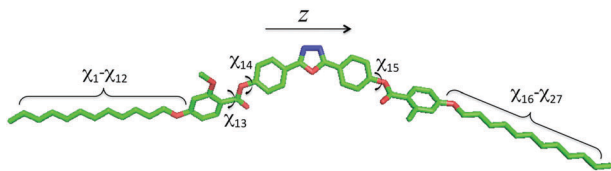
Fig. 3 Molecular structure of compound 1 without hydrogen atoms. Arrows show the dihedral ( \chi_i ) allowed to rotate in the Monte Carlo conformation sampling. The molecular frame \{x, y, z\} has the z axis passing through the carbon atoms of the oxadiazole ring and y perpendicular to the plane of the ring.
