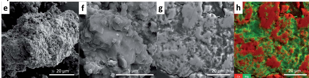
Fig. 5 SEM micrographs of CO 2 cycled mined dolomite (Watheroo, Wath-D-cat, (a–d)) and synthetic dolomite (Synth-D-cat, (e–h)) with secondary electron (SE) or backscattered electron detectors (BSE). (a/e) Typical conglomerated particle (SE), (b/f) higher magnification image of the particle surface (BSE) (c/g) polished cross-section of a powder grain (BSE), (d/h) EDS elemental map of an epoxy embedded cross section (coloured elemental maps overlaid onto BSE image, colour legend in the image).
