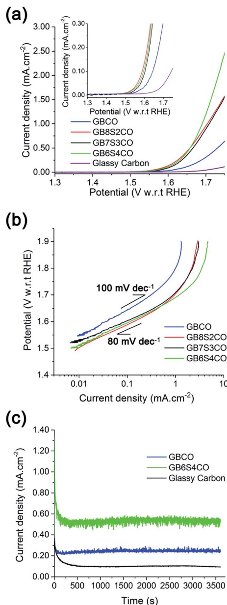
Fig. 9 (a) Linear sweep voltammetry at the 6 th cycle and the corresponding (b) Tafel plot (at 1 mV s -1 scan rate) in 0.1 M KOH electrolyte. (c) Chronoamperometry measurements of different GBSCO compounds at 1.65 V ( \eta = 420 mV). Electrochemical measurements were iR compensated using current interrupt method. Higher performance was achieved with higher Sr dopant level.
