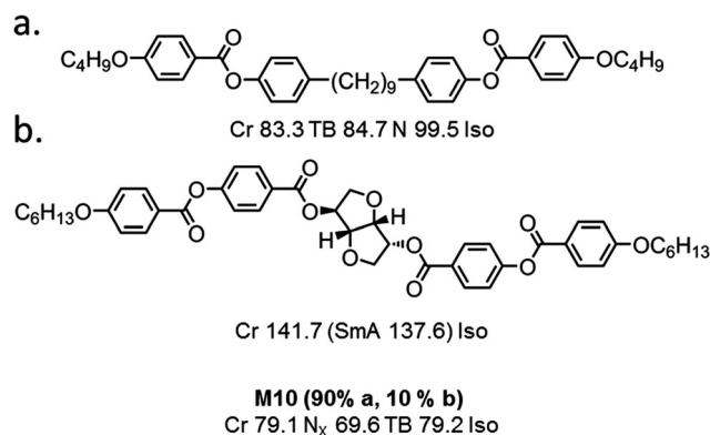
Fig. 1 Molecular structures and transition temperatures ( ^{\circ}C ) of CA23 (a) and RM1041 (b). The composition and transition temperatures of the mixture 'M10' are indicated.
