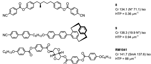
Fig. 6 Molecular structures, transition temperatures (°) and helical twist-ing power values (HTP, \mu\text{m}^{-1} ) for the three chiral dopants used.
