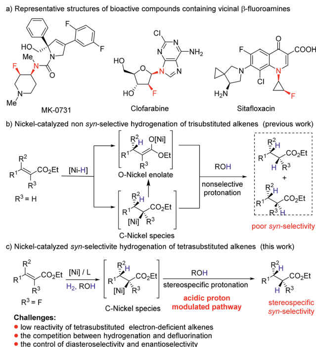
Fig. 1 Ni-catalyzed asymmetric hydrogenation of olefins.
