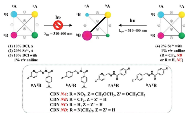
Scheme 3 Weighted graph representation of modifications of the four [2 × 2] CDNs of the four constituents PA a B, bA 1 B, PA h B and bA h B (3.5 mM each) under light irradiation (λ irr = 310–400 nm) starting from the statistical distribution in the presence of a different catalyst and temperature conditions. (Top left) No photoselection takes place with catalysts (1)–(3). (Top right) the system undergoes photoselection in the case of NB and NC in the presence of the combined catalysts (4). PA h B exists in both E and Z isomers. The diagonal and edges of the square link agonistic (+) and antagonistic (–) constituents, respectively. See Tables S1–S4† for numerical values.
