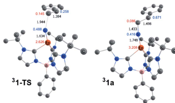
Fig. 7 Optimized structures with selected bond distances in Å of 31-TS and 3a . Black values indicate bond lengths in Å, red values indicate \alpha Mulliken spin densities, and blue values are excess \beta spin densities.
