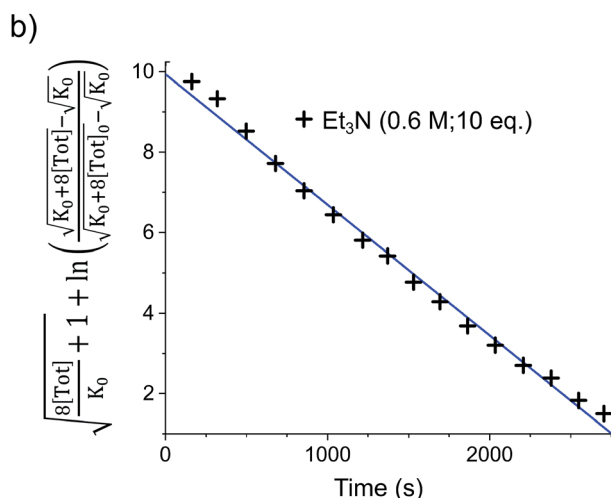
Fig. 3 (a) Solutions of 1 (0.03 mmol) in d_8 -toluene (0.5 mL) under \text{H}_2 (4 bar) containing various base concentrations were prepared. When the stannylenic concentration, [\text{Tot}] , is plotted against the normalised timescale t \cdot [\text{Et}_3\text{N}]^1 , all traces overlap, confirming the order in base to be one. (b) Linearised rate data for a similar solution of 1 (0.03 mmol) in d_8 -toluene (0.5 mL) under \text{H}_2 (4 bar) containing \text{Et}_3\text{N} (0.6 M; 10 eq.).
