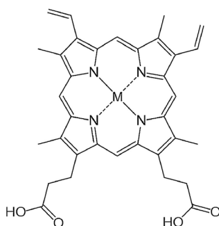
Fig. 8 Chemical structure of metalloprotoporphyrins (MPP). Reprinted with permission from ref. 126. Copyright 2017, Elsevier.
