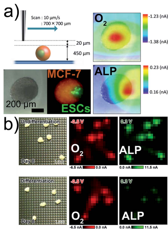
Fig. 4 (a) SECM, optical, and fluorescence imaging of a co-culture Janus spheroid fused on day 3 ( 250^{\text{ESC}}-2000^{\text{MCF-7}} ). Respiration activity (O 2 ) imaging at -0.5 V and ALP activity imaging at +0.3 V. (b) Electrochemical imaging of O 2 and ALP activities of EBs. All potentials vs. Ag/AgCl. Adapted with permission from ref. 7 and 57. Copyright (a) 2013 and (b) 2017 American Chemical Society.
