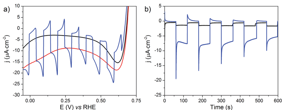
Fig. 11 (a) LSVs at the NiOIRBG-174I \text{Co}_{\text{C11P}} electrode with (red line), without (black line) or with chopped (blue line) light irradiation recorded at a scan rate of 10 \text{ mV s}^{-1} and (b) current densities vs. time at NiOIRBG-174I \text{Co}_{\text{C11P}} (blue line) and NiOIRBG-174I \text{Co}_{10\text{P}} (black line) electrodes poised at 0.14 V vs. RHE under chopped light irradiation, in MES 0.1 M/NaCl 0.1 M aqueous electrolyte at pH 5.5.
