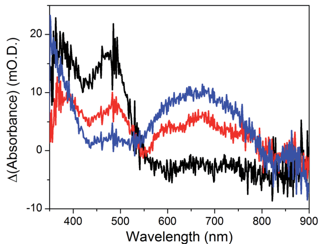
Fig. 10 Differential UV-visible spectra recorded at a NiOIRBG-174I \text{Co}_{\text{C11P}} electrode poised at -0.4 V vs. Ag/AgCl ( -0.3 V vs. NHE, black line) with subtraction of the spectrum of the same electrode poised at 0 V vs. Ag/AgCl ( +0.1 V vs. NHE taking into account interliquid junction potential 45 ), -0.7 V vs. Ag/AgCl ( -0.6 V vs. NHE, blue line) with subtraction of the spectrum of the same electrode poised at -0.4 V vs. Ag/AgCl and -0.4 V vs. Ag/AgCl ( -0.3 V vs. NHE) under light irradiation (red line) with subtraction of the spectrum of the same electrode poised at -0.4 V vs. Ag/AgCl in the dark, in \text{CH}_3\text{CN} n\text{Bu}_4\text{NPF}_6 0.1 M electrolyte.
