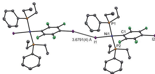
Fig. 2 Molecular structure of 2pl showing intermolecular C–I...Ni halogen bond. Displacement ellipsoids at 50% probability level. Hydrogen atoms not shown. A three-molecule chain is illustrated in the ESI.†
