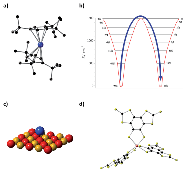
Fig. 5 (a) Molecular structure of [\text{Dy}(\text{Cp}^{\text{ttt}})_2]^+ , where \text{Cp}^{\text{ttt}} = \{\text{C}_5\text{H}_2^t\text{Bu}_3\text{-}1,2,4\} and ^t\text{Bu} = \text{C}(\text{CH}_3)_3 . H atoms are omitted for clarity. Dy: blue and C: black. (b) Energy levels and M_J projections of [\text{Dy}(\text{Cp}^{\text{ttt}})_2]^+ , determined by CASSCF-SO calculations. (c) Ho atom on a MgO monolayer. Mg: yellow and O: red. (d) Molecular structure of [\text{V}(\text{C}_8\text{S}_8)_3]^{2-} . V: red, C: black, and S: yellow.
