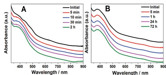
Fig. 4 Thermostability of \text{Au}_{42}(\text{TBBT})_{26} (A) and \text{Au}_{44}(\text{TBBT})_{28} (B).
