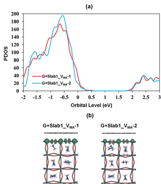
Fig. 18 (a) Calculated partial density of states (PDOS) of MAPbI 3 in the V MA -containing graphene + MAPbI 3 hybrids, and (b) the orbital shape of the valence band edges of MAPbI 3 (isovalence: 0.015 a.u.).
