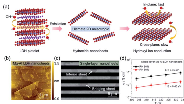
Fig. 5 (a) Schematic drawings of the structure of the LDH platelet, ultimate single-layer nanosheets and hydroxyl ion conduction. (b) AFM characterization of single-layer Mg-Al LDH nanosheets. (c) SEM characterization of single-layer Mg-Al LDH nanosheets deposited on comb electrodes. (d) Temperature-dependent in-plane hydroxyl ion conductivities of single-layer Mg-Al LDH nanosheets at 50% and 80% RH. Reproduced with permission. 31 Copyright 2017, The American Association for the Advancement of Science.
