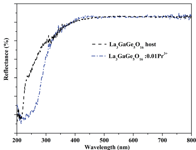
Fig. 2 (a) Diffuse reflectance spectra of pure \text{La}_3\text{GaGe}_5\text{O}_{16} and \text{La}_3\text{GaGe}_5\text{O}_{16}:0.01\text{Pr}^{3+} at room temperature.
