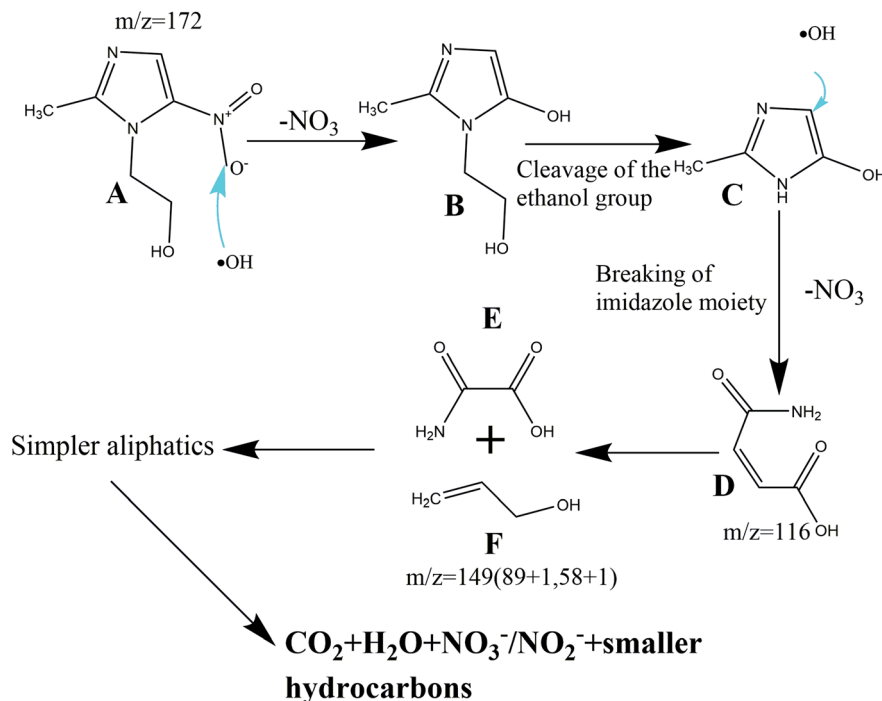
Scheme 2 Proposed MNZ degradation and mineralization pathway by Fe/Si codoped \text{TiO}_2 .
