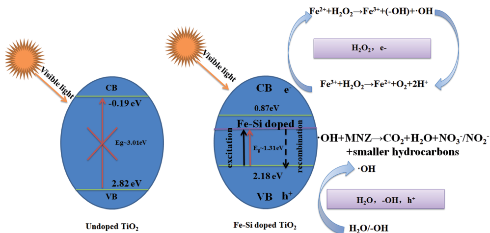
Scheme 3 Proposed mechanism for MNZ degradation with Fe/Si codoped \text{TiO}_2 under visible light irradiation.
