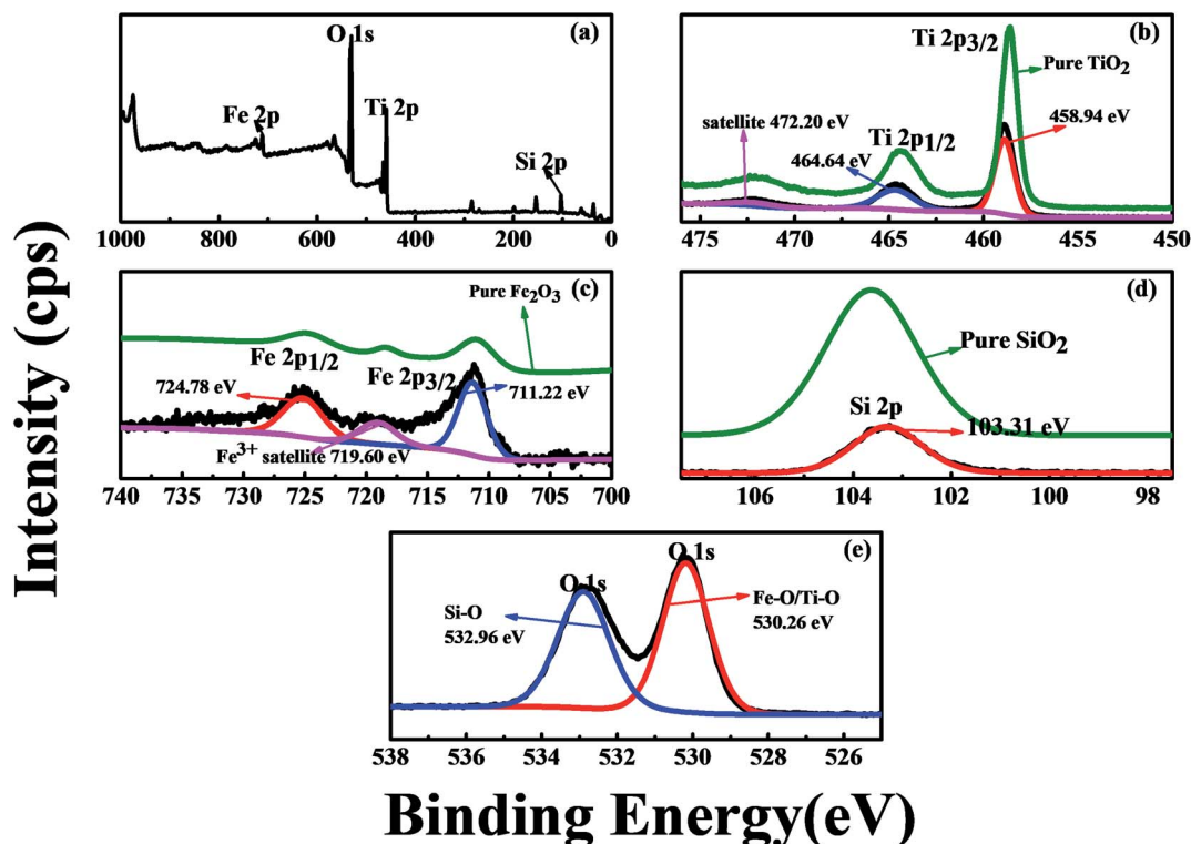
Fig. 5 XPS spectra of Fe/Si codoped \text{TiO}_2 . (a) Survey; (b) Ti 2p peaks; (c) Fe 2p peaks; (d) Si 2p peak; (e) O 1s peaks.
