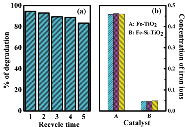
Fig. 10 (a) Reusability of Fe/Si codoped TiO 2 for degradation of MNZ. (b) The concentrations of iron ions in MNZ solution after degradation using Fe doped TiO 2 and Fe/Si codoped TiO 2 .
