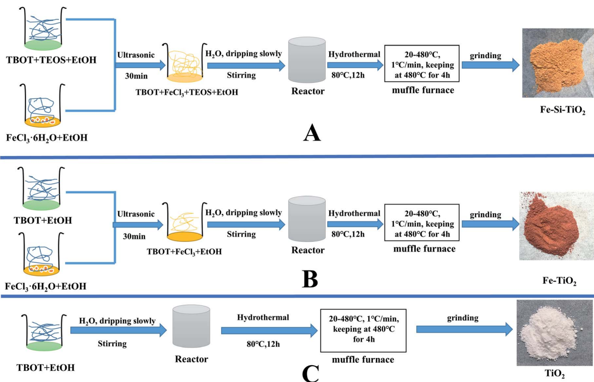
Scheme 1 Schematic route for synthesizing Fe/Si codoped \text{TiO}_2 , Fe doped \text{TiO}_2 and \text{TiO}_2 ((A) Fe/Si codoped \text{TiO}_2 , (B) Fe doped \text{TiO}_2 and (C) \text{TiO}_2 ).
