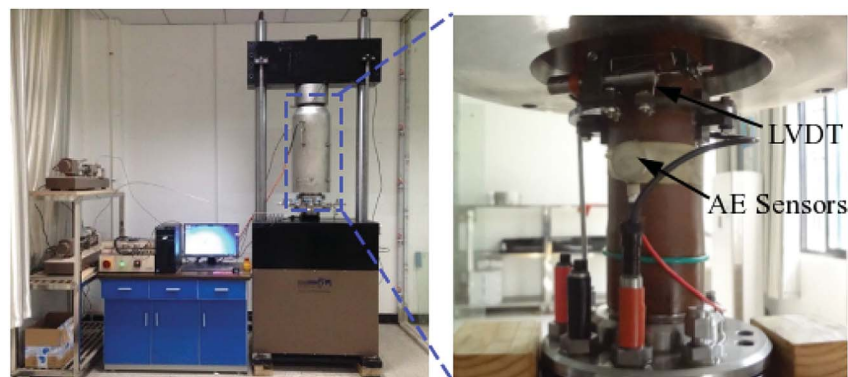
Fig. 2 Illustration of the test equipment.
