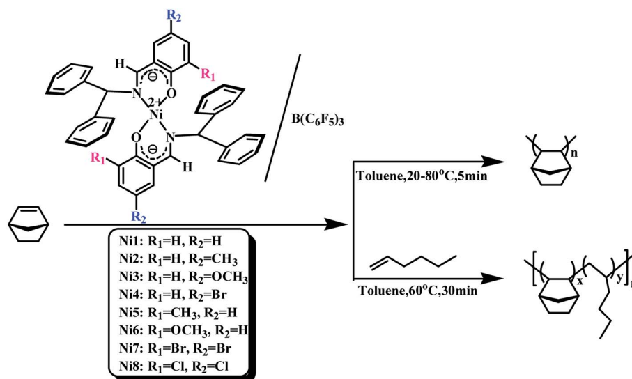
Scheme 2 Norbornene homopolymerization catalysed by Ni1–Ni8/ \text{B}(\text{C}_6\text{F}_5)_3 and copolymerization of norbornene and 1-hexene catalyzed by Ni1 and Ni2/ \text{B}(\text{C}_6\text{F}_5)_3 .
