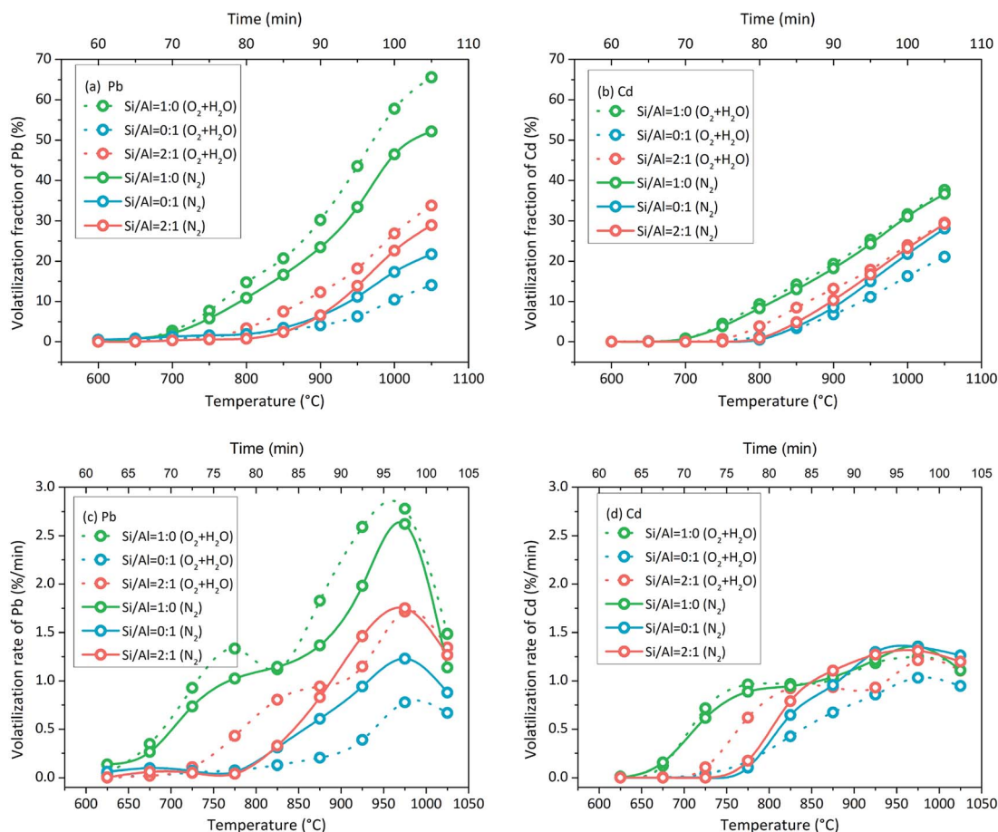
Fig. 5 Accumulative volatilization fractions of (a) Pb and (b) Cd and volatilization rates of (c) Pb and (d) Cd with increasing temperature in 85% O 2 + 15% H 2 O atmosphere and N 2 atmosphere.
