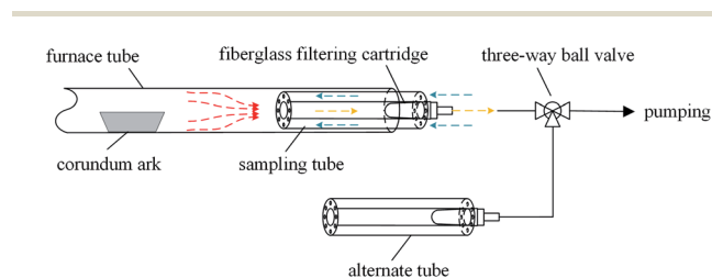
Fig. 1 Heavy metal sampling device.
