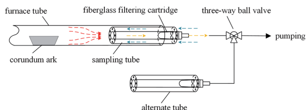
Fig. 1 Heavy metal sampling device.
