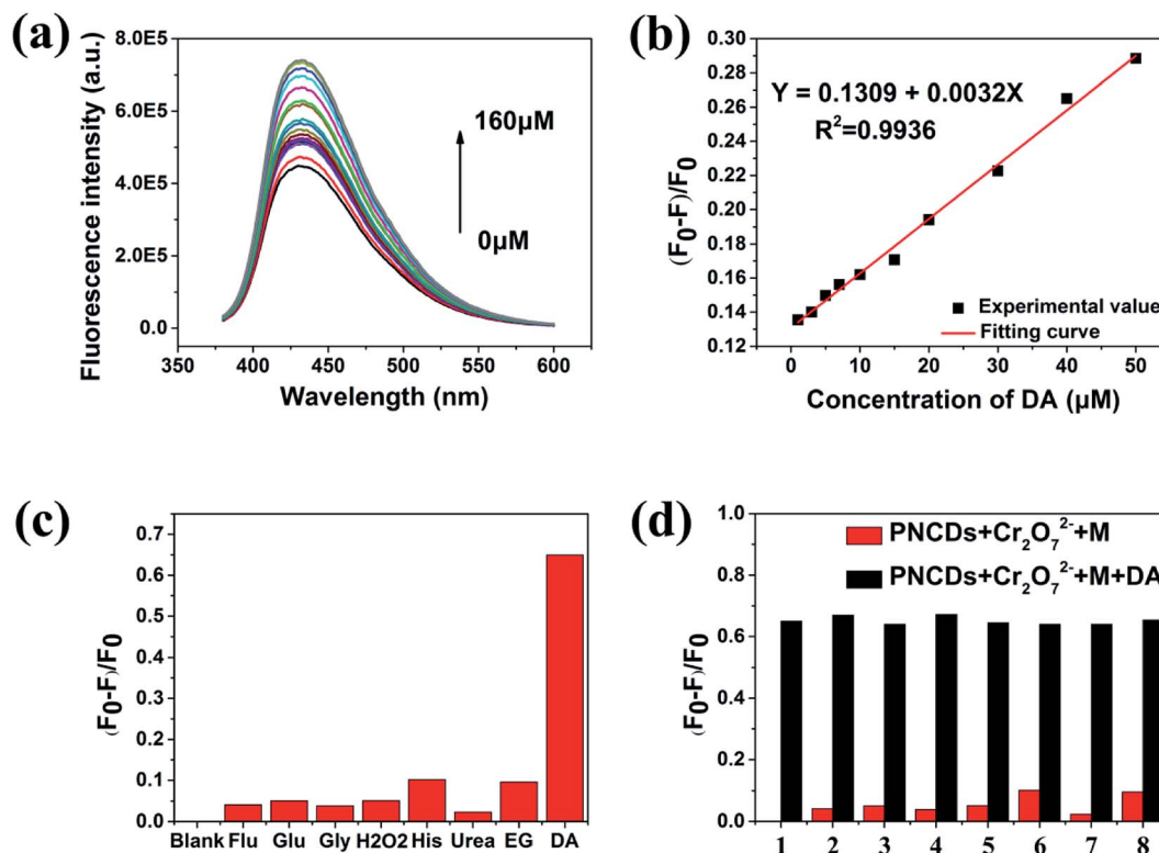
Fig. 5 (a) Fluorescence recovery of the PNCd/Cr(VI) mixture to DA at various concentrations (0, 0.5, 1, 3, 5, 7, 10, 15, 20, 30, 40, 50, 70, 90, 100, 120, 140, 150, 160 \mu\text{mol L}^{-1} ). (b) Plot of the (F_0 - F)/F_0 with the concentration of DA. (c) and (d) (F_0 - F)/F_0 of the PNCd in PBS (pH: 7.4) with 160 \mu\text{M} different reducing biomolecules. F and F_0 correspond to the fluorescence intensities of the PNCd without and with 160 \mu\text{M} of different reducing biomolecules (the numbers 1 to 8 are corresponding to blank, Flu, Glu, Gly, \text{H}_2\text{O}_2 , His, urea, EG, respectively).
