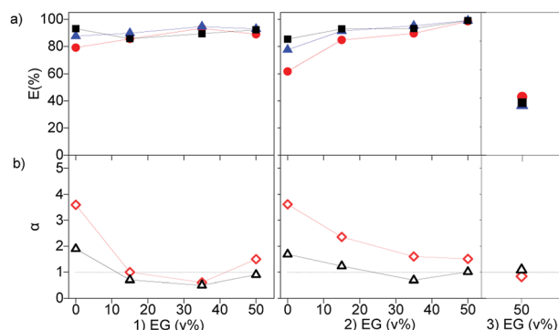
Fig. 6 (a) Extraction of La (●), Ce (▲) and Pr (■), and (b) separation factors of \alpha_{La}^{Pr} (◇) and \alpha_{Ce}^{Pr} (Δ) as a function of ethylene glycol (EG) in the feed solution. One contact with (1) 10 wt% Cy923 in [A336][NO 3 ], (2) 10 wt% Cy923 in [C101][NO 3 ] and (3) pure [C101][NO 3 ]. At 80 °C, 3000 rpm, volume O/A 1 : 1. Chloride feed solution: 1.7, 4.0, 0.6 g L -1 of La(III), Ce(III) and Pr(III), 2 mol L -1 CaCl 2 .
