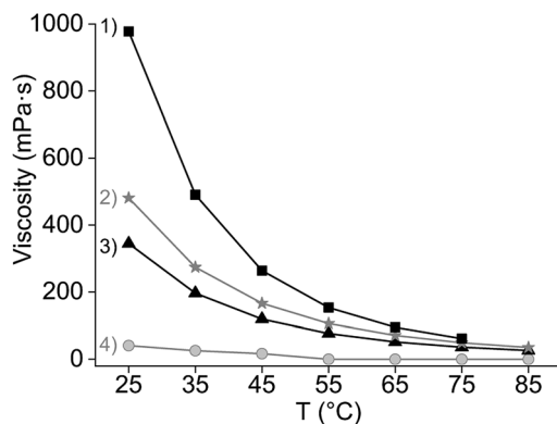
Fig. 5 Viscosity as a function of the temperature and the organic phase composition: (1) pure Cy923, (2) 20 v% Cy923 in [C101][NO 3 ], (3) 10 wt% Cy923 in [C101][NO 3 ] and (4) pure [C101][NO 3 ]. At 80 °C, 3000 rpm, volume O/A 1 : 1. Chloride feed solution: 1.7, 4.0, 0.6 g L -1 of La(III), Ce(III) and Pr(III), 2 mol L -1 CaCl 2 .
