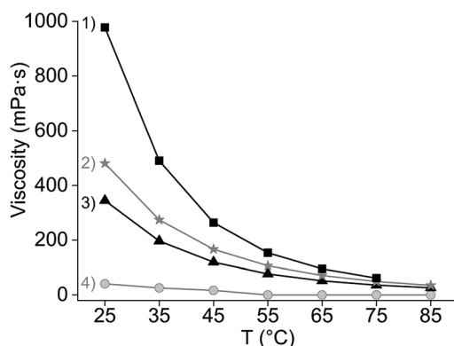
Fig. 5 Viscosity as a function of the temperature and the organic phase composition: (1) pure Cy923, (2) 20 v% Cy923 in [C101][NO 3 ], (3) pure [C101][NO 3 ] and (4) after loading 39 g L -1 of REE in 20 v% Cy923 in [C101][NO 3 ].
