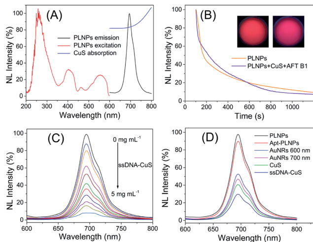
Fig. 2 (A) Excitation and emission spectra of PLNPs and absorption spectra of CuS nanoparticles. (B) Afterglow property of PLNPs and PLNPs-CuS nanoprobe in the presence of AFT B1. (C) The luminescence quenching of CuS NPs to PLNPs. (D) Comparison of the quenching effect of AuNRs and CuS NPs on the luminescence of PLNPs.
