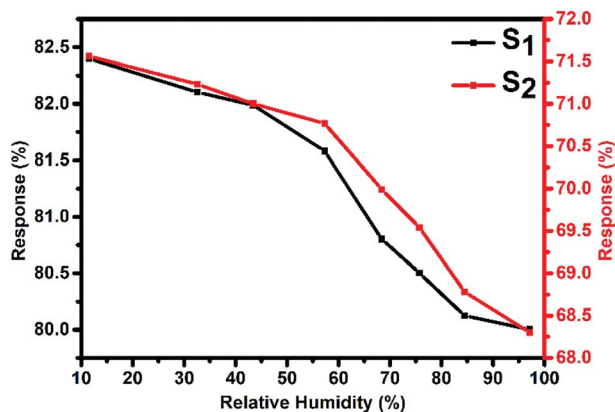
Fig. 10 Variation in the Cl 2 response of S 1 and S 2 sensors with humidity for 2 ppm of Cl 2 at room temperature.
