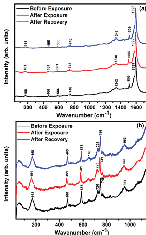
Fig. 12 Raman spectra of the S 2 sensor recorded (a) before exposure (black curve); after exposure (red curve) to 25 ppm of Cl 2 and after full recovery (blue curve) (b) in the range 30–1300 cm -1 (magnified view).
