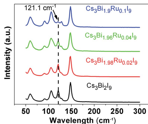
Fig. 4 Raman spectra of the \text{Cs}_3\text{Bi}_{2-x}\text{Ru}_x\text{I}_9 ( x = 0, 0.02, 0.04 , and 0.1 ) samples.
