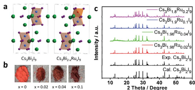
Fig. 1 (a) Crystal structure of Cs 3 Bi 2 I 9 and Cs 3 Bi 2-x Ru x I 9 . (b) Photos of samples synthesized in this work showing darkened colour with increasing Ru 3+ doping. (c) Powder XRD of Cs 3 Bi 2 I 9 and Cs 3 Bi 2-x Ru x I 9 with x = 0.02, 0.04, 0.1, 0.2.
