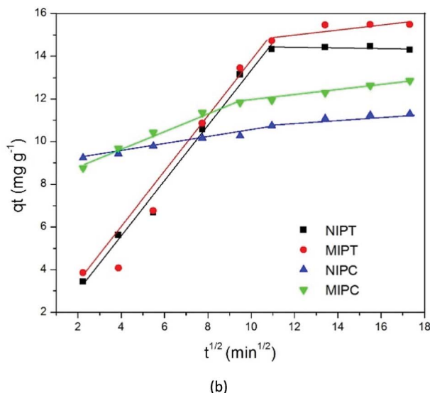
Fig. 4 Kinetic models (a) and intraparticle diffusion (b) of the polymers.
