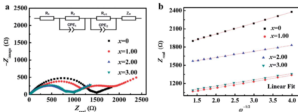
Fig. 6 (a) EIS Nyquist plots of NCMO- x wt% \text{CeO}_2 ( x = 0, 1.00, 2.00 and 3.00 ) composites and the equivalent circuit in inset, and (b) their linear fitting of the Z_{\text{real}} versus \omega^{-1/2} .
