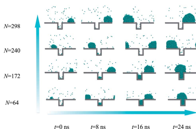
Fig. 8 Droplet nucleation and growth on the rough surface for four sizes of initial existing droplet.
