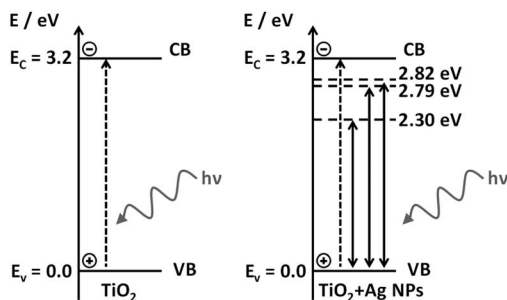
Scheme 3 Band diagram of \text{TiO}_2 and \text{TiO}_2 + \text{Ag NPs} samples.
