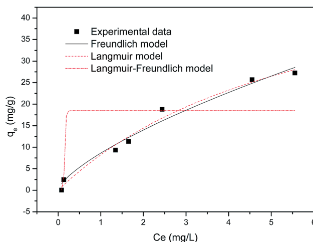
Fig. 4 Adsorption isotherm curves of DMP on biochar.
