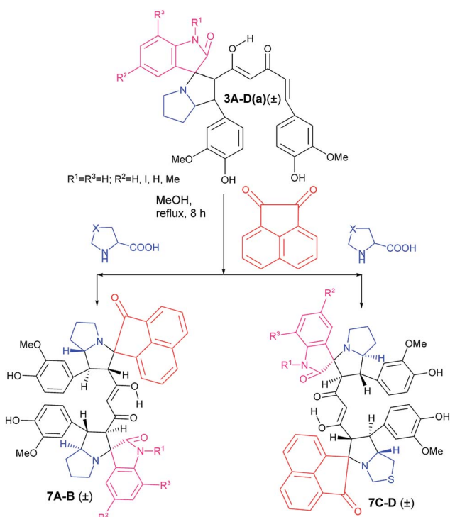
Scheme 4 Synthesis of mixed bis-pyrrolizidino/-thiopyrrolizidino dispiro-oxindolo-acenaphthylino curcuminoids.
