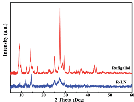
Fig. 3 XRD patterns of rufigallol and R-LN.
