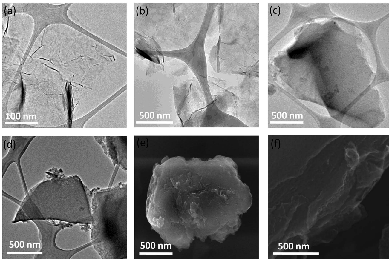
Fig. 6 (a and b) HRTEM image of (\text{BN})_{0.3}\text{C}_{0.7} , (c and d) TEM image of BCN with cross-linking of graphene-graphene domains ( \text{GG}/(\text{BN})_{0.3}\text{C}_{0.7}-\text{BN}_{0.3}\text{C}_{0.7} ), (e) SEM image of \text{GG}/(\text{BN})_{0.3}\text{C}_{0.7}-\text{BN}_{0.3}\text{C}_{0.7} , (f) BCN with cross-linking of graphene-BN/ (\text{BN}) domains ( \text{GBN}/\text{GG})_{0.3}\text{C}_{0.7}-\text{BN}_{0.3}\text{C}_{0.7} ).
