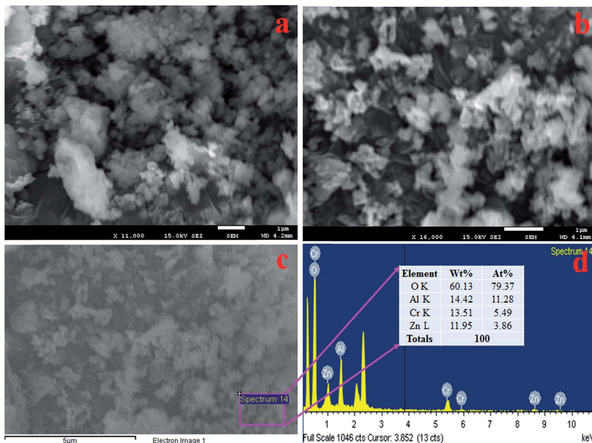
Fig. 3 Structural and compositional analysis of the prepared \text{ZnO}/\text{Al}_2\text{O}_3/\text{Cr}_2\text{O}_3 NPs. (a and b) Low and high magnification FESEM images and (c and d) elemental analysis with EDS.
