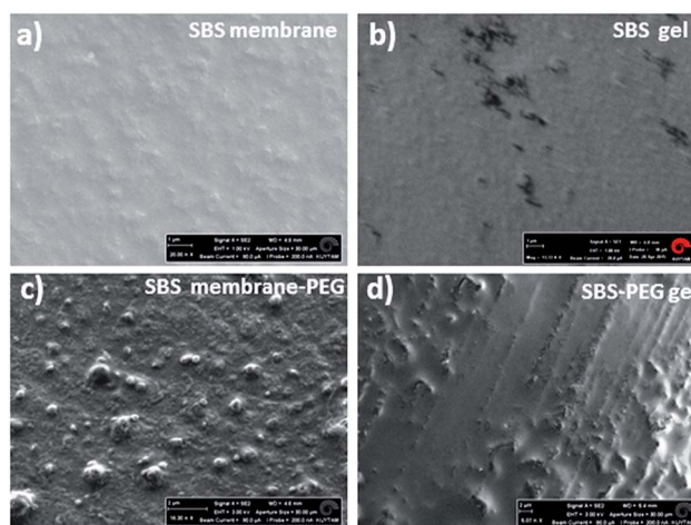
Fig. 5 SEM images of (a) SBS membrane (scale bar 1 μm) (b) SBS gel (scale bar 1 μm) (c) SBS membrane-PEG (scale bar 2 μm) and (d) SBS-PEG gel (scale bar 2 μm). SBS membrane-PEG gels were prepared by casting SBS solution after incorporation of PEG particles. SBS gel and SBS-PEG gel were prepared by crosslinking of SBS solution after incorporation of PEG particles. Hybrid gels were dried in vacuum oven overnight before analysis with SEM.
