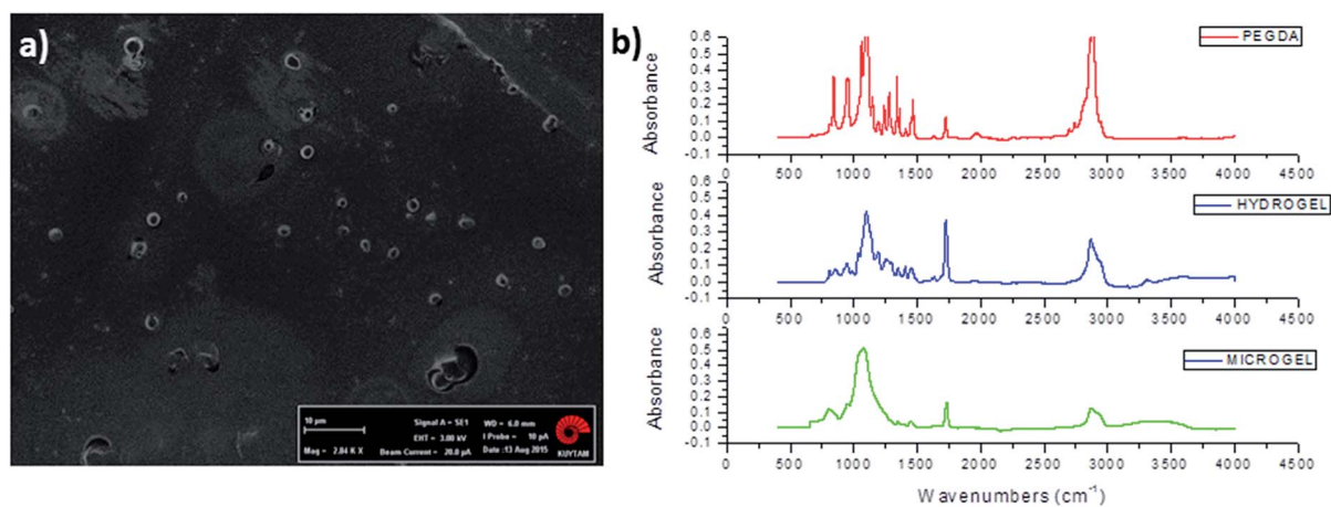
Fig. 3 Structural characterization of PEG particles. (a) SEM image of casted PEG particles (scale bar: 10 μm) (b) FTIR spectra of PEGDA, PEG bulk hydrogel and PEG microgel.
