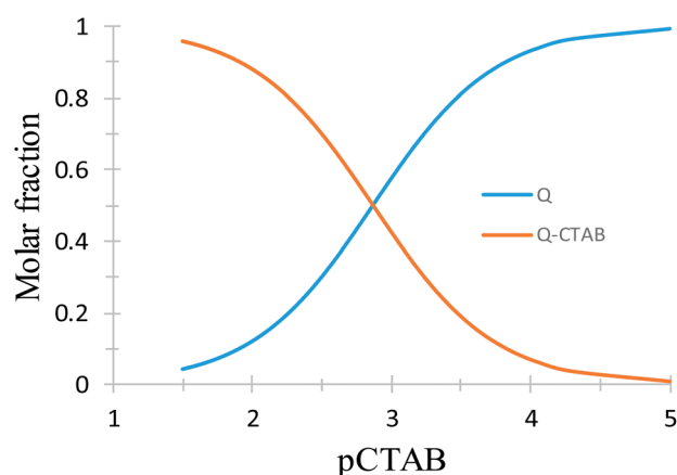
Fig. 3 Distribution diagram of the quercetin, Q, species as a function of pCTAB = -\log[CTAB] .
