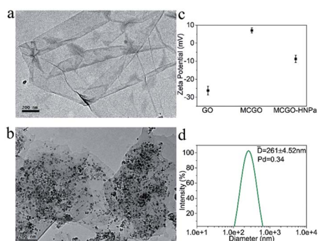
Fig. 1 TEM images of GO (a) and magnetic chitosan/graphene oxide composite MCGO (b); (c) zeta potential of GO, MCGO and MCGO–HNPs in ethanol solutions of pH = 7.0. (d) Hydrodynamic size distribution of MCGO–HNP measured by dynamic light scattering (DLS).
