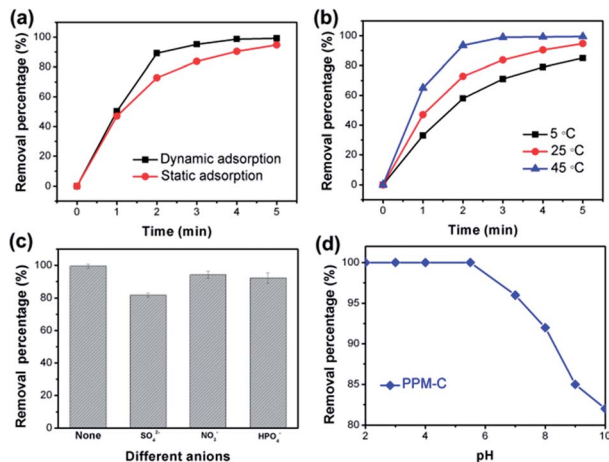
Fig. 8 (a) The Cr(vi) RP of PPM-C vs. time under dynamic adsorption (100 rpm) and static adsorption at room temperature (25 °C), (b) the Cr(vi) RP of PPM-C vs. time at different temperature (under static adsorption), (c) effect of competing anions, and (d) solution pH on the Cr(vi) RP of PPM-C (the concentration of SO 4 2- (Na 2 SO 4 ), NO 3 - (NaNO 3 ), and H 2 PO 4 - (KH 2 PO 4 ) is 0.01 M). (PPM-C for the Cr(vi) removal at different conditions is PP15-M1.5-C).
