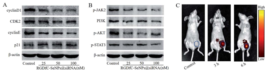
Fig. 6 (A) The protein expression levels of cyclin D1, CDK2, cyclin E and p21 in HepG2 cells treated with different concentrations of RGDfC-SeNPs@siRNA were detected via western blotting. (B) The protein expression levels of p-JAK2, PI3K, p-AKT and p-STAT3 in HepG2 cells treated with different concentrations of RGDfC-SeNPs@siRNA were detected via western blotting. (C) In vivo fluorescence images of mice after injecting with RGDfC-SeNPs@cy5.5-siRNA for 3 or 6 h; mice receiving no injection formed the control group.
