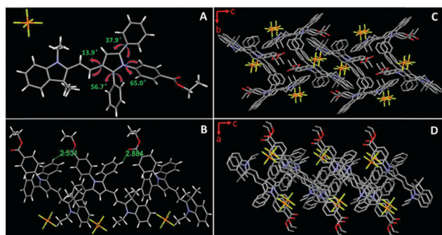
Fig. 3 Single crystal structure of TPP-1 (CCDC 1853627 † ): (A) molecular structure, (B) intermolecular interactions, and (C and D) molecular packing mode (hydrogen omitted for clarity).
