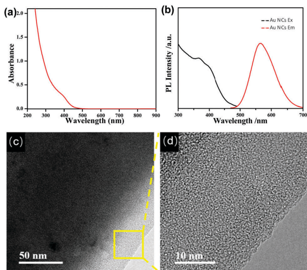
Fig. 1 UV-vis absorption spectrum (a), photoexcitation ( \lambda_{em} = 565 nm, black line) and photoemission ( \lambda_{ex} = 365 nm, red line) spectra of the Au NCs (b). (c) TEM image of the Au NCs at pH 2.0. (d) HRTEM image of the zone marked by the yellow frame in (c).
