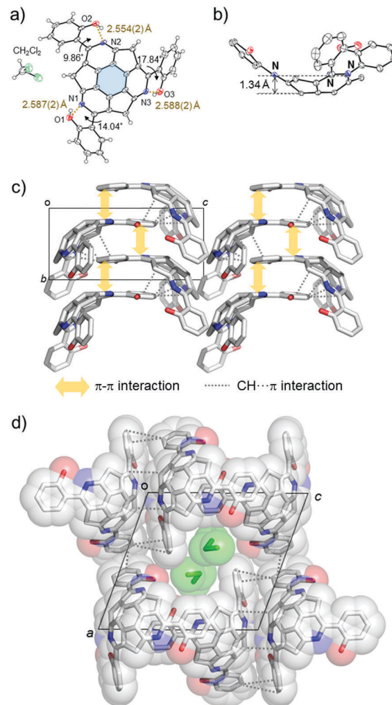
Fig. 2 Crystal structure of ( A )-(+)- 1 . (a) ORTEP model of ( A )-(+)- 1 . The brown dotted lines show the intramolecular hydrogen bonds. (b) The deepest position of the bowl depth. In (a and b), the ellipsoids are shown in 50% probability. (c) Stacking structure viewed from the b axis with intermolecular \pi - \pi (yellow solid arrow) and CH... \pi (grey dotted line) interactions. (d) One-dimensional channel structure with intercolumnar CH... \pi interactions. Green molecules correspond to the encapsulated CH 2 Cl 2 . The colour codes in each of the images in this figure are: C, grey; N, blue; O, red; Cl, light green; however, (e) in (a), the hydrogen atoms are omitted for clarity.
