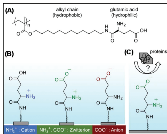
Fig. 20 (A) Chemical structure of PGluDMA. (B) pH-Responsiveness of the glutamic acid in the polymer side chains exposed to the polymer film/water interface. (C) Unknown protein adsorption behavior of the zwitterionic state on the polymer film at neutral pH. Reproduced with permission from ref. 187. Copyright (2015) The Royal Society of Chemistry.
