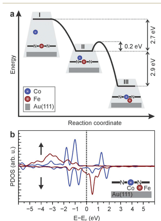
Fig. 3 DFT calculations. (a) Calculated reaction barriers of (I) initial, (II) intermediate, and (III) final state of the transmetalation. (b) Projected density of states onto Fe and Co d-orbitals in the final state.
