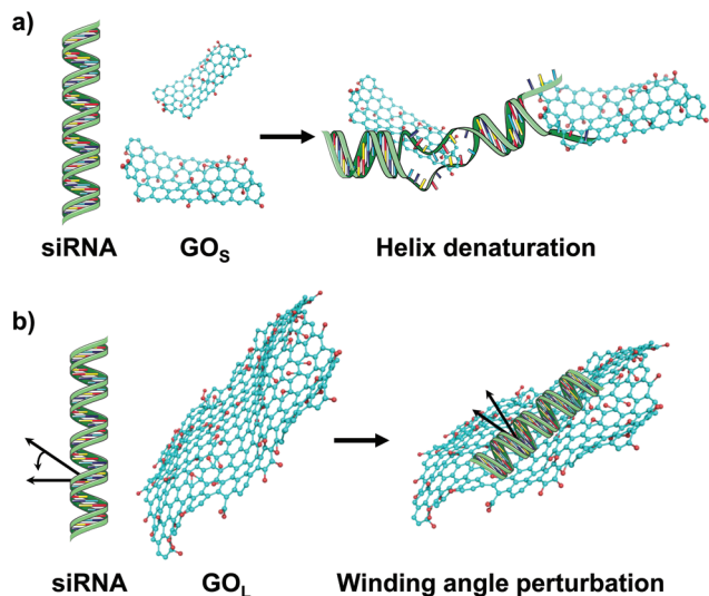
Fig. 5 Cartoon illustrating the possible interactions and conformational changes of (a) \text{GO}_\text{S} and (b) \text{GO}_\text{L} with the siRNA molecule.
