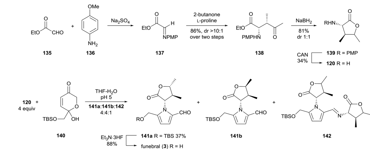
Scheme 10 Synthesis of funebral (3) by Brimble and co-workers.
