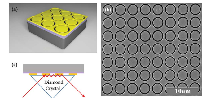
Fig. 1 (a) Schematic diagram of the metasurface design on the \text{SiO}_2/\text{Si} substrate; (b) top-view SEM image of a 50\ \text{nm} -thick metasurface deposited on the substrate; (c) a schematic illustration of the ATR sampling technique in the measurement.
