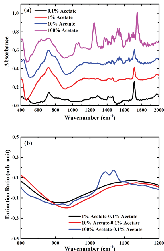
Fig. 5 (a) Measured absorption spectra of mixtures in the presence of metasurface on Si substrate in the ambient atmosphere, spectra are consecutively shifted by 0.2 vertically for clarity; (b) zoomed extinction spectra of mixtures in the presence of metasurface on Si substrate for the carbon–oxygen stretching band region between 800\text{ cm}^{-1} and 1200\text{ cm}^{-1} .
